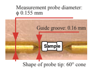
SMD TEST FIXTURE IM9110 Direct connection two-terminal measurement type for measuring SMDs, DC to 1 MHz, measurable sample sizes: 008004 (EIA)
