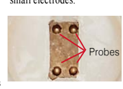
SMD TEST FIXTURE 9699 Direct connection type, For measuring SMDs with electrodes on the bottom; DC to 120 MHz, test sample dimensions: 1.0 mm (0.04 in) to 4.0 mm (0.16 in) wide, max. 1.5 mm (0.06 in) high
