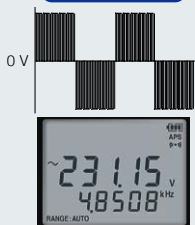
Typical waveform + harmonic components
